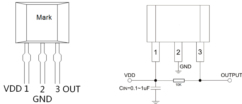
TO-92S
