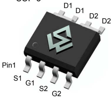
SOP-8
