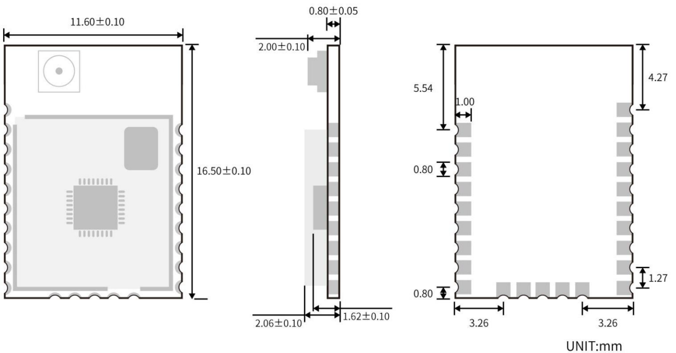
RF-BM-BG22A1/A2/A3I 尺寸图
